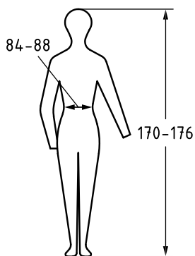
Figure D.2 — Minimum requirements for trousers
