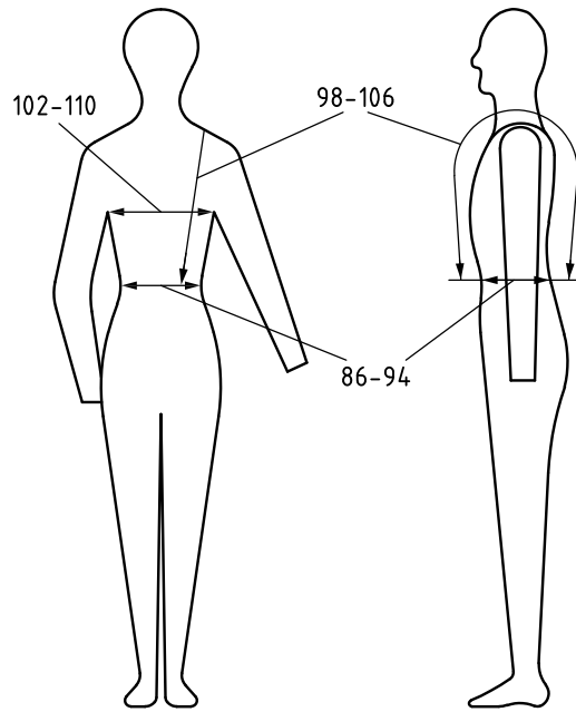
Figure D.4 — Torso protector for men
